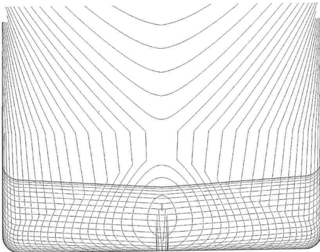
BODY PLAN
