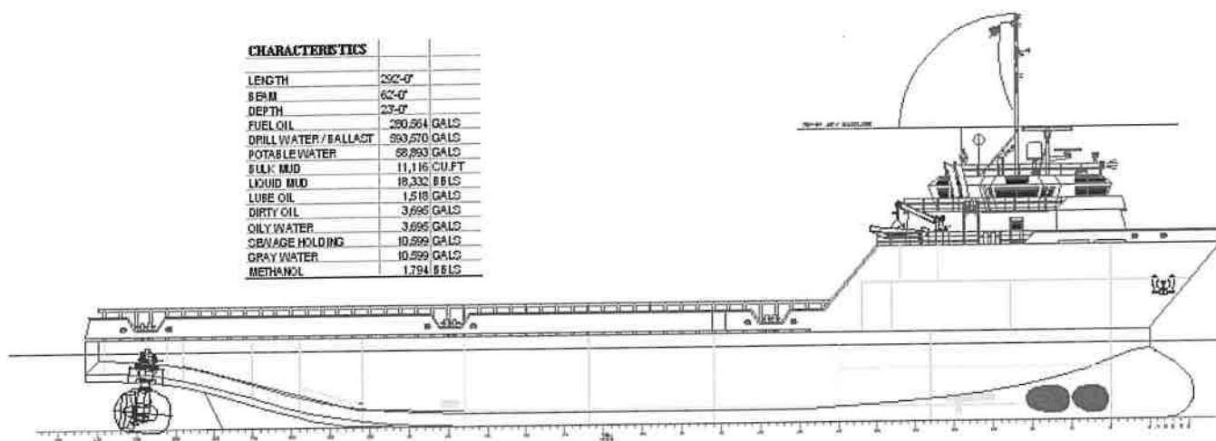
OUTBOARD PROFILE
